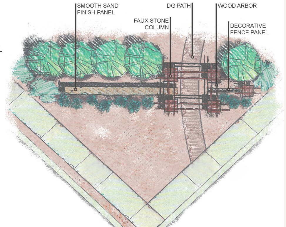
PLAN - PRIMARY ENTRY MONUMENT
