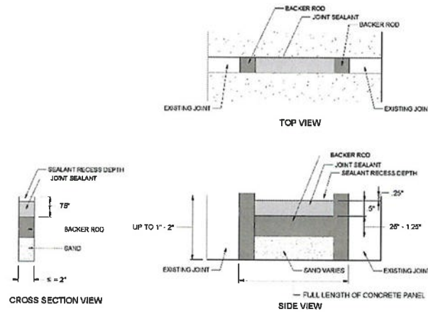
EXPANSION JOINT CROSSING BACKER ROD
