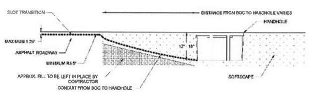
SINGLE POINT ENTRY INTO TRADITIONAL SOFTSCAPE (ASPHALT)
