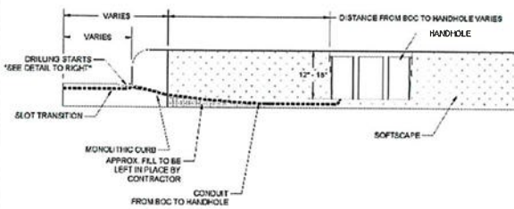
SINGLE/MID-SPAN POINT ENTRY INTO TRADITIONAL HANDHOLE SOFTSCAPE
