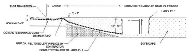
SINGLE POINT ENTRY INTO TRADITIONAL SOFTSCAPE (CONCRETE DRAINAGE CURB)
