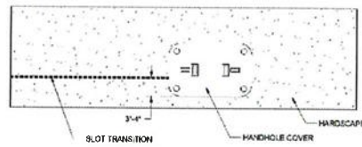
SINGLE POINT ENTRY INTO TRADITIONAL HANDHOLE HARDSCAPE
