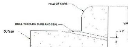
SINGLE POINT ENTRY INTO TRADITIONAL HANDHOLE CURB-SOFTSCAPE
