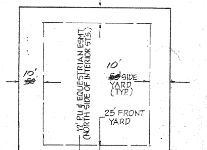
TYPICAL SETBACKS & EASEMENTS N.T.S.
