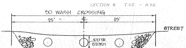
TYPICAL CULVERT & DIP SECT. AT WASH CROSSING
